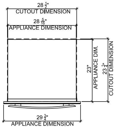
1 PLAN
