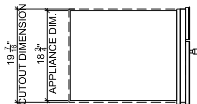
3 SIDE ELEVATION
