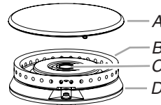
A. Burner cap B. Burner head C. Gas opening D. Burner base
