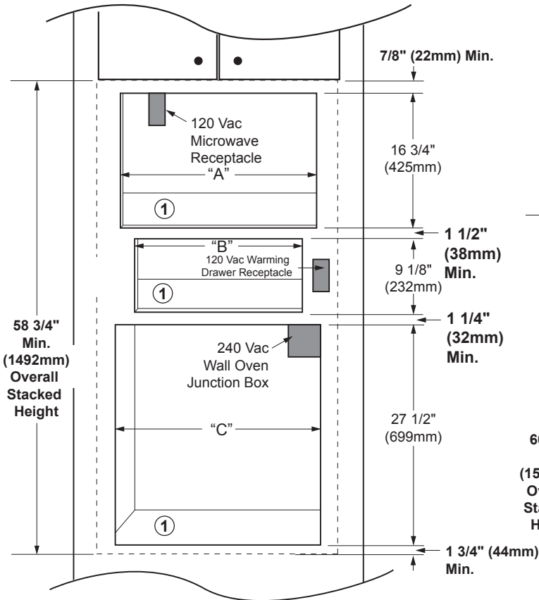
CUTOUT DIMENSIONS DMT2420 SHOWN
