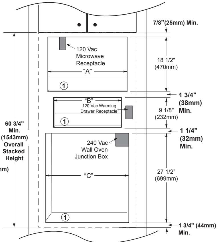
CUTOUT DIMENSIONS DCM24 SHOWN
