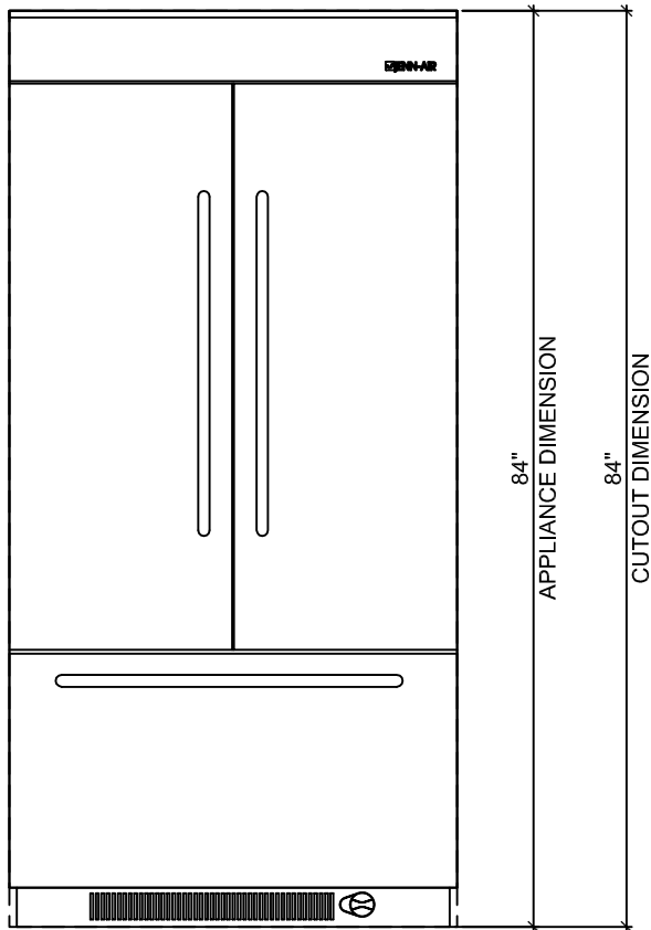
2 FRONT ELEVATION
