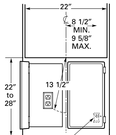
Recommended Main Shut-Off Location (The regulator also has a shut-off lever)
