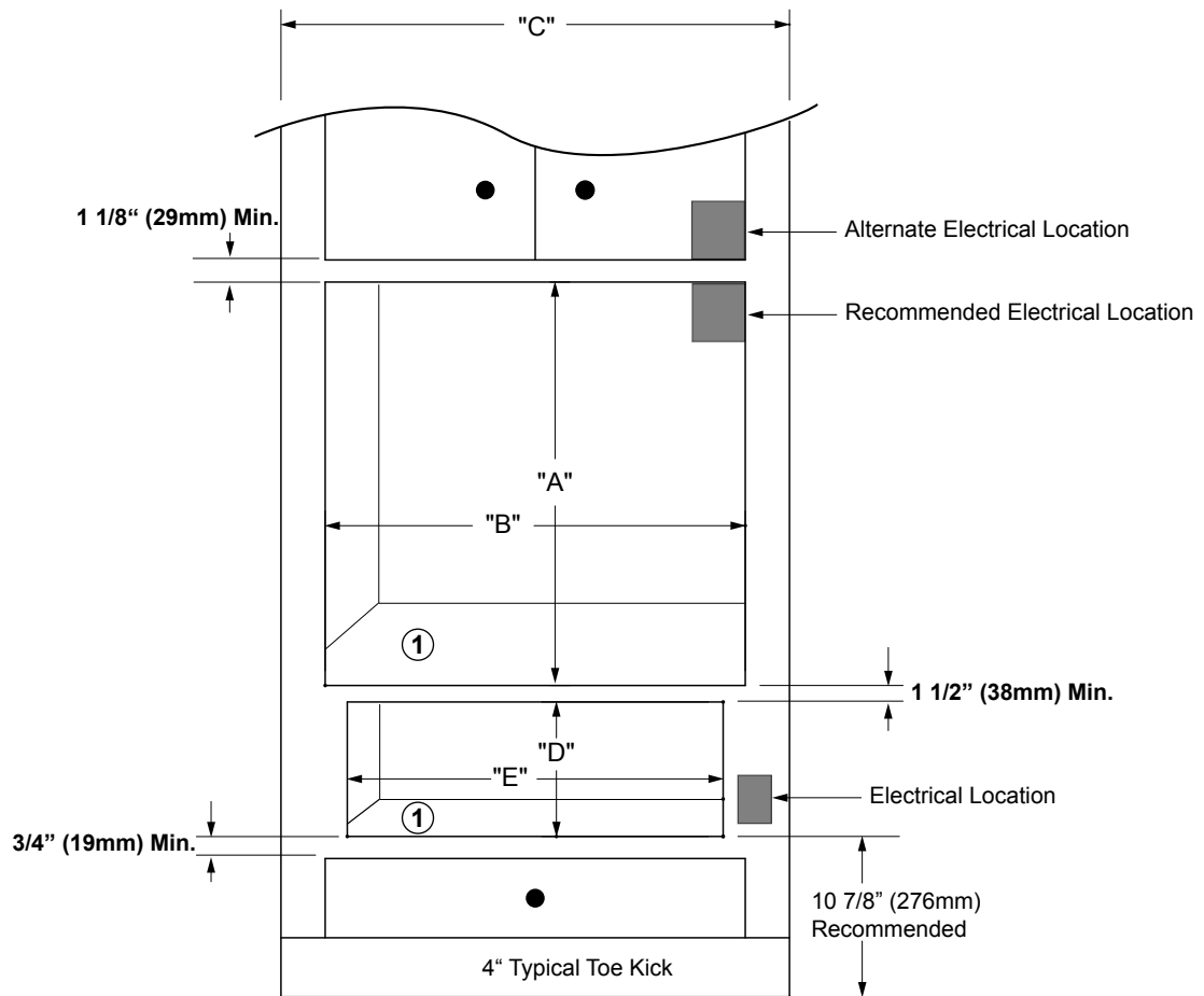
SINGLE WALL OVEN, WARMING OVEN STACKED CUTOUT DIMENSIONS
