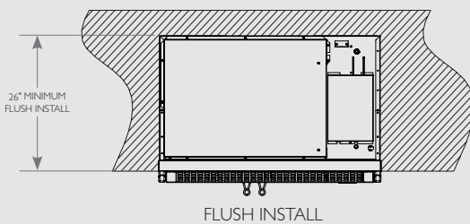
TOP VIEW FIGURE 1 - ROUGH OPENING
