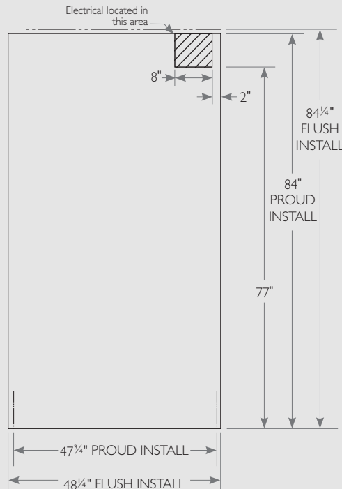
FRONT VIEW FIGURE 2 - ROUGH OPENING
